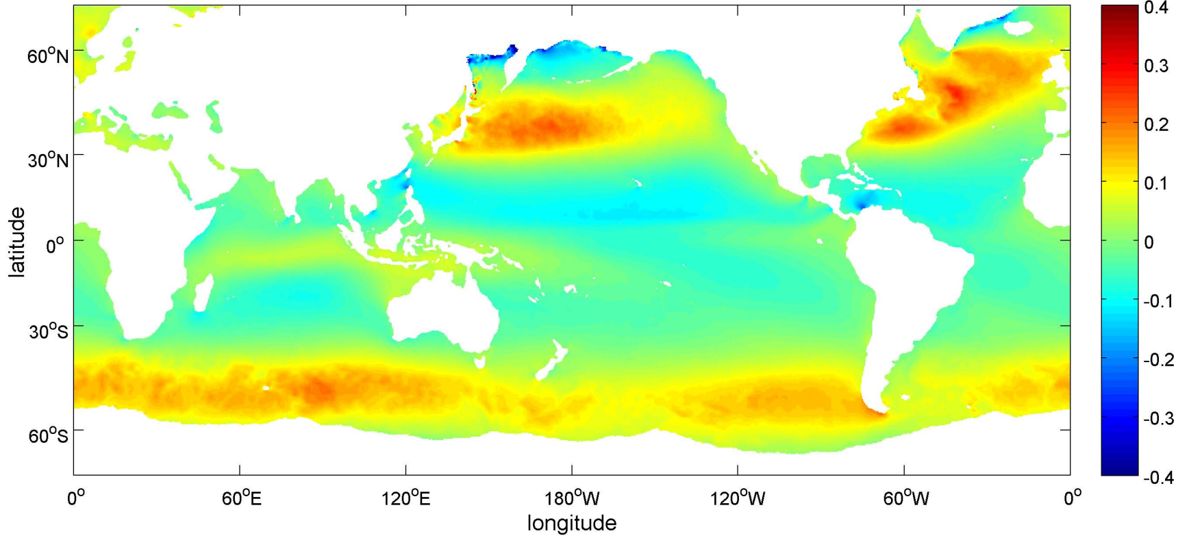
SCOW January Zonal Wind Stress ( \text{N/m}^2 )
