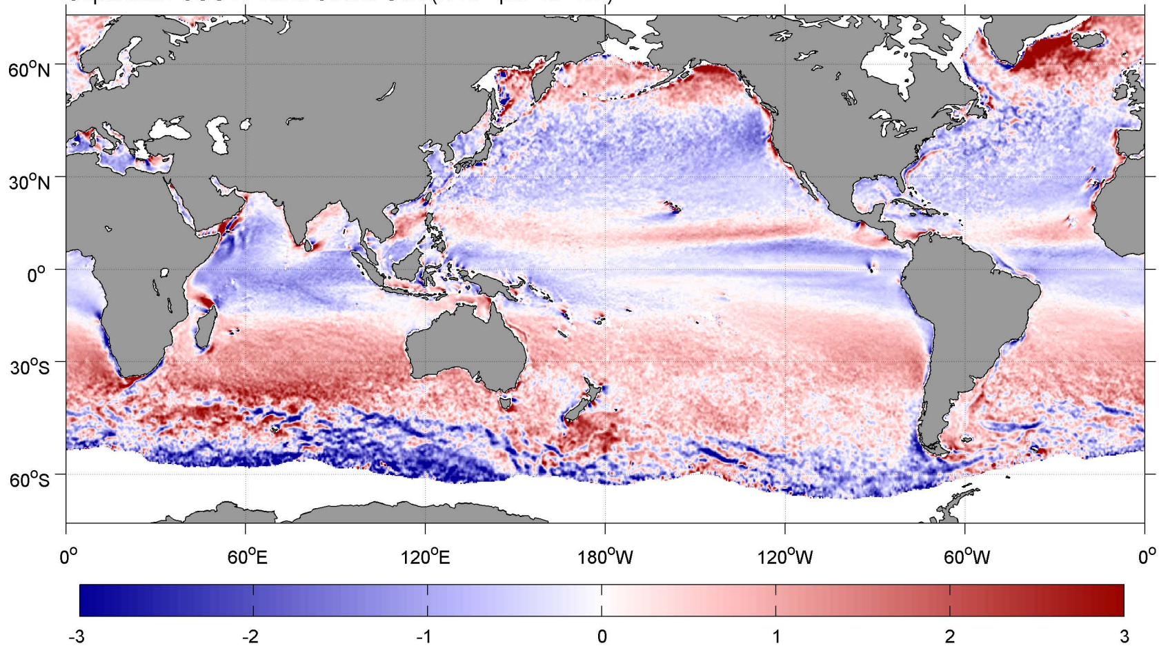
September SCOW Wind Stress Curl ( \text{N m}^{-2} per 10^4 \text{ km}^2 )
