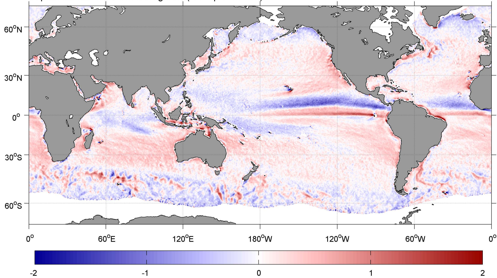
September SCOW Wind Divergence ( \text{m s}^{-1} per 10^2 \text{ km} )
