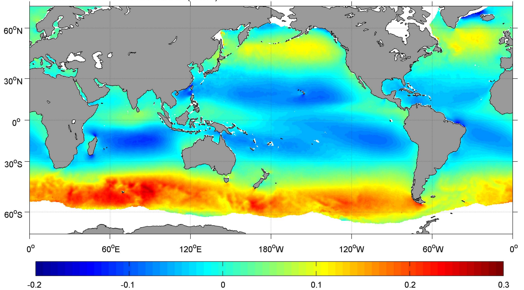
October SCOW Zonal Wind Stress ( \text{N m}^{-2} )
