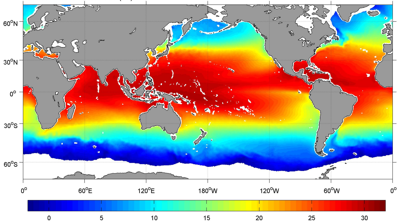
October SCOW AMSR SST ( ^{\circ}\text{C} )
