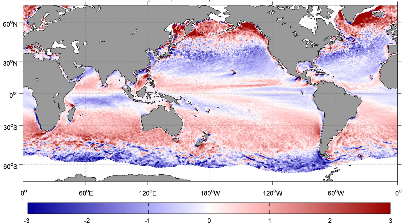
November SCOW Wind Stress Curl ( \text{N m}^{-2} per 10^4 \text{ km}^2 )
