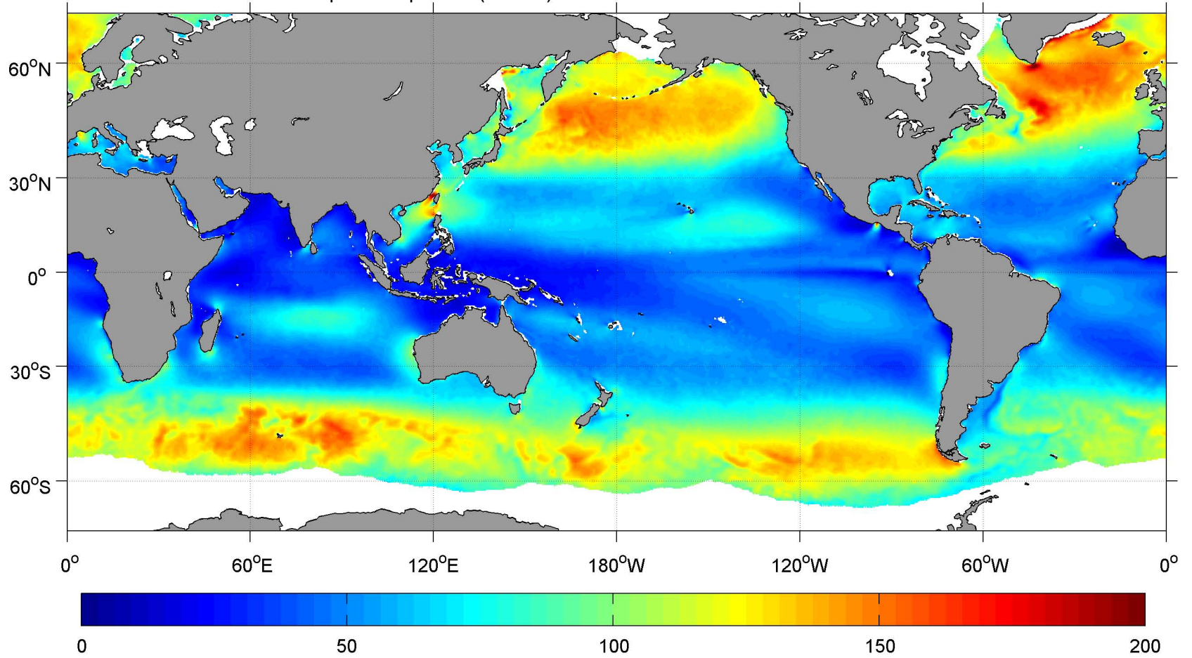
November SCOW Wind Speed Squared ( \text{m}^2 \text{s}^{-2} )
