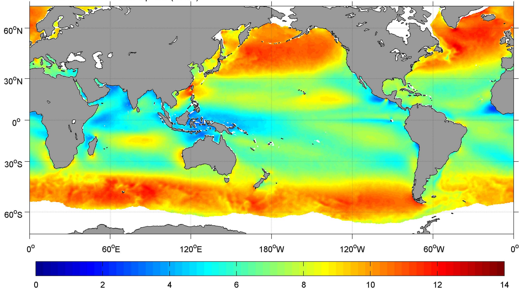
November SCOW Wind Speed ( \text{m s}^{-1} )
