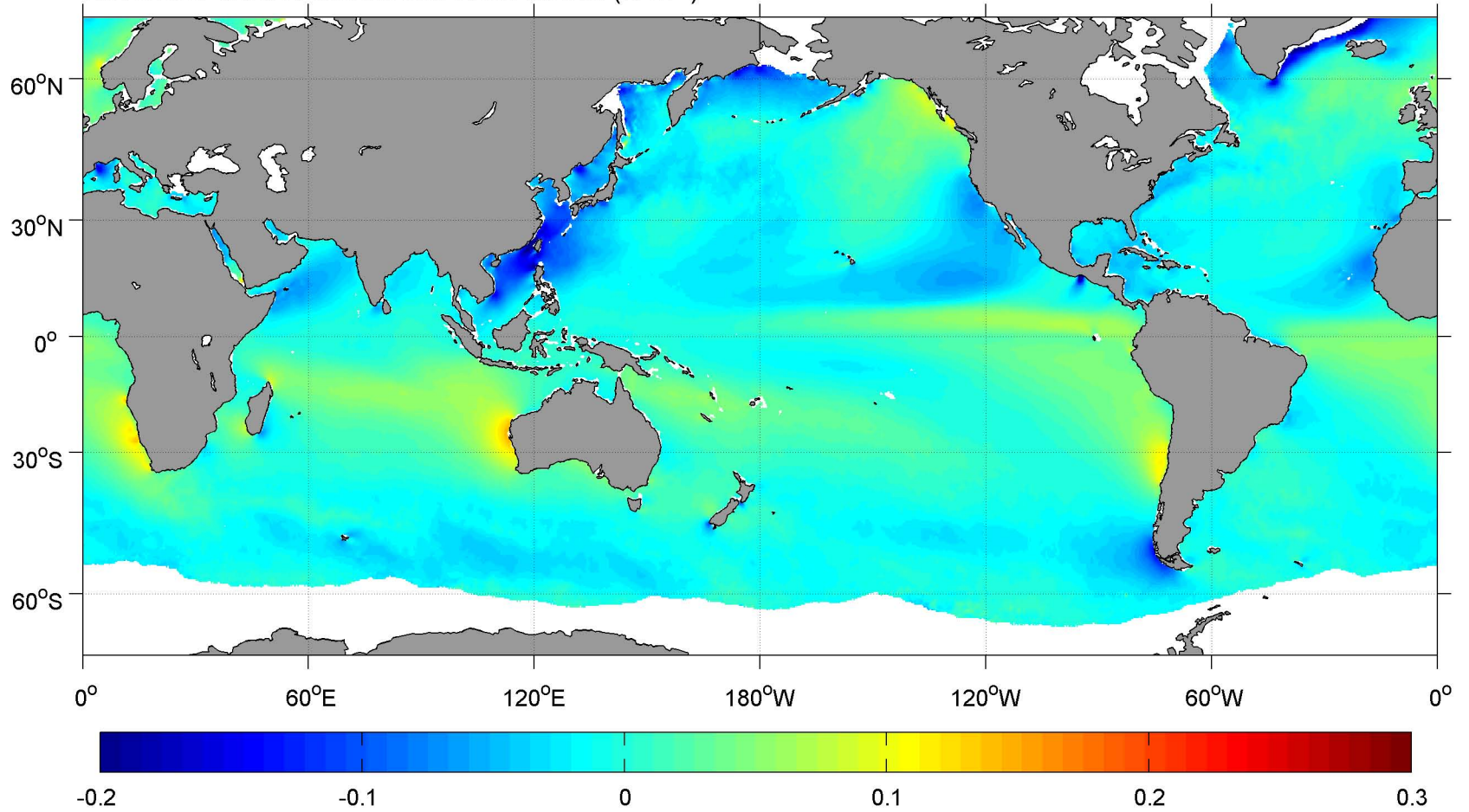
November SCOW Meridional Wind Stress ( \text{N m}^{-2} )
