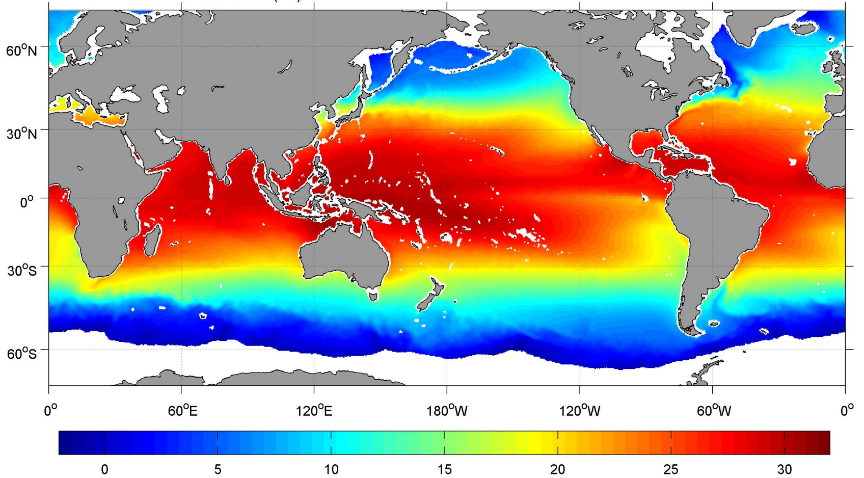
November SCOW AMSR SST ( ^{\circ}\text{C} )
