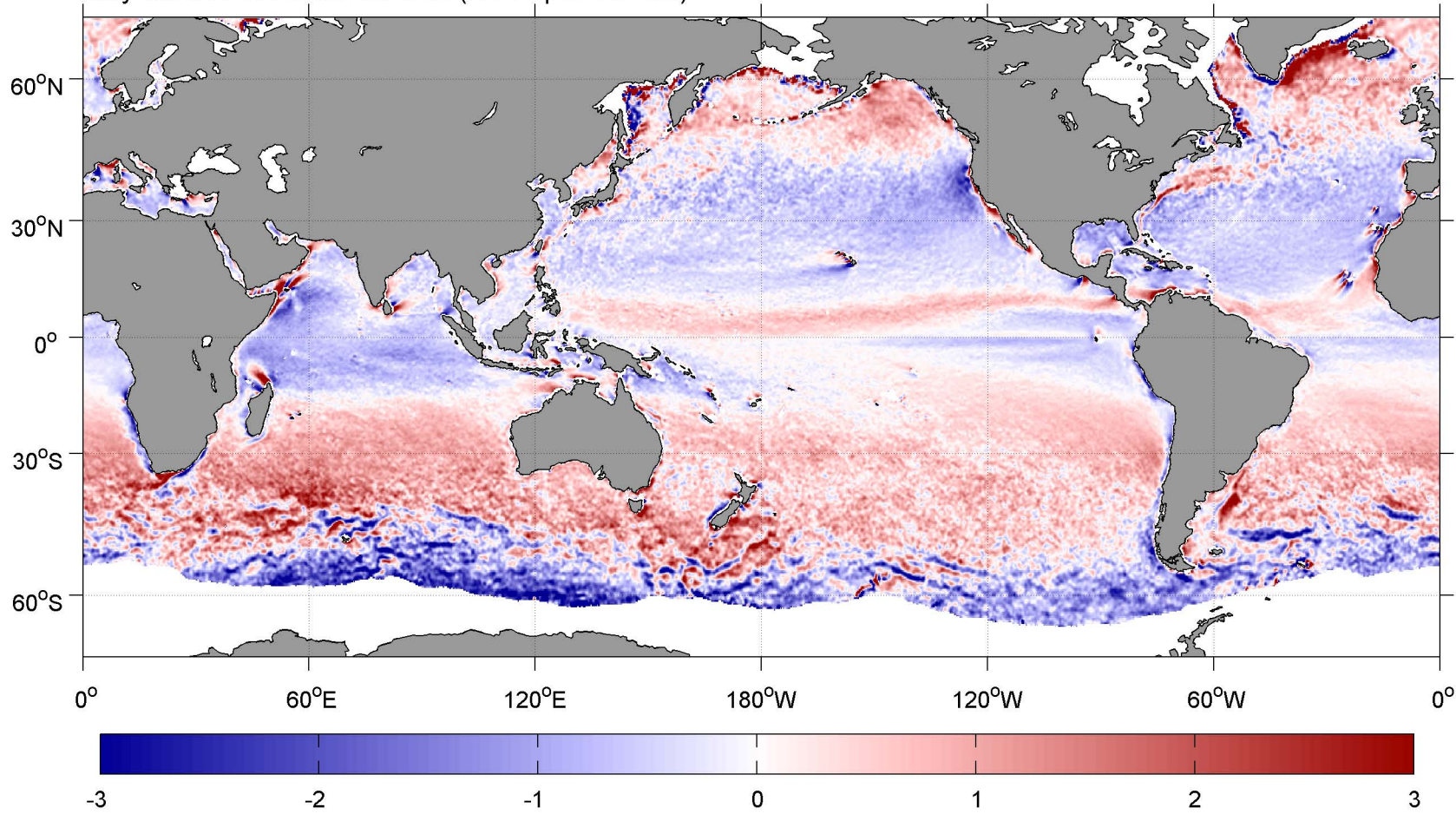
May SCOW Wind Stress Curl ( \text{N m}^{-2} per 10^4 \text{ km} )
