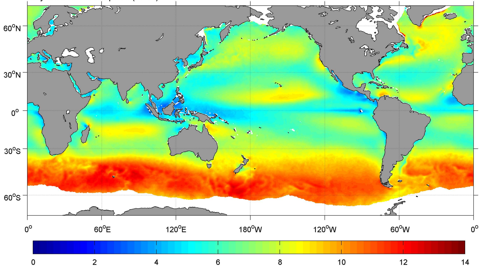
May SCOW Wind Speed ( \text{m s}^{-1} )
