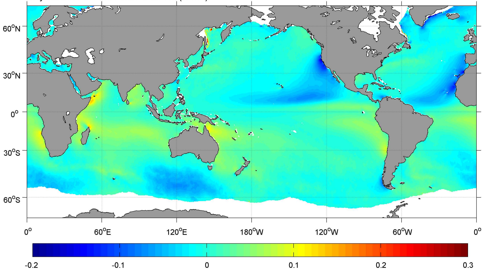
May SCOW Zonal Meridional Stress ( \text{N m}^{-2} )
