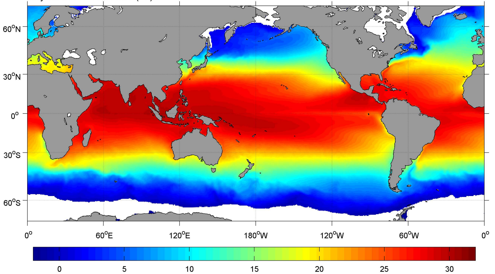
May SCOW AVHRR SST ( ^{\circ}\text{C} )
