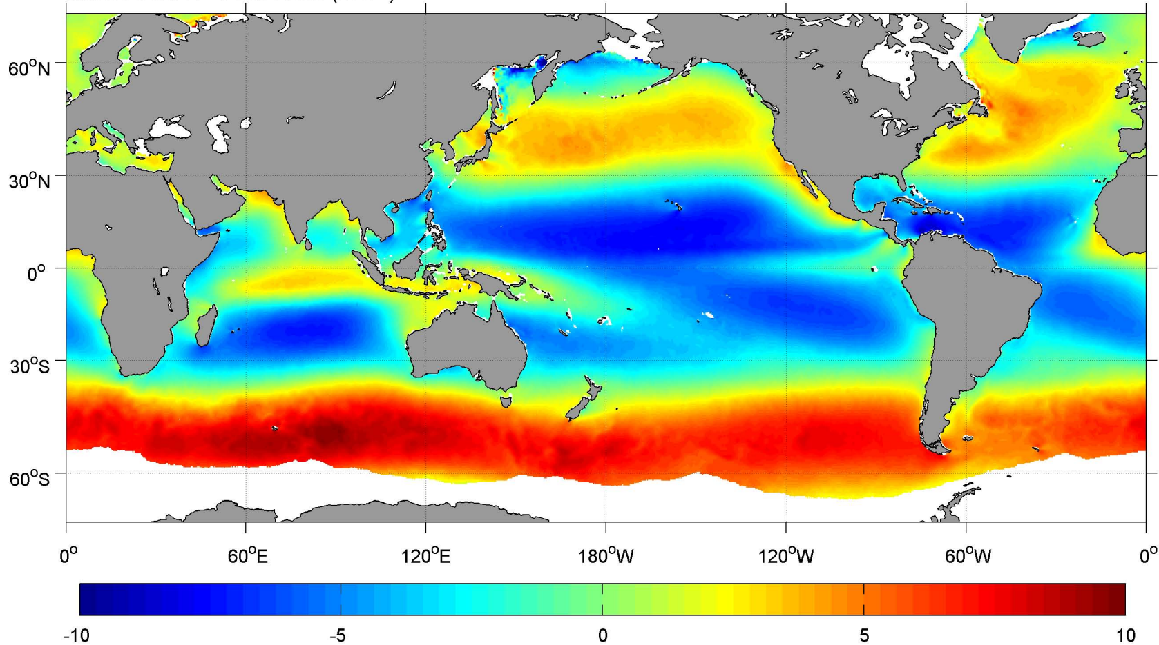
March SCOW Zonal Wind ( \text{m s}^{-1} )
