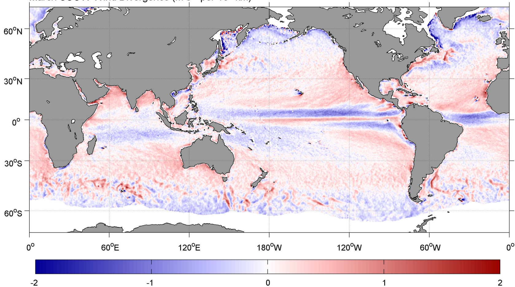
March SCOW Wind Divergence ( \text{m s}^{-1} per 10^2 \text{ km} )
