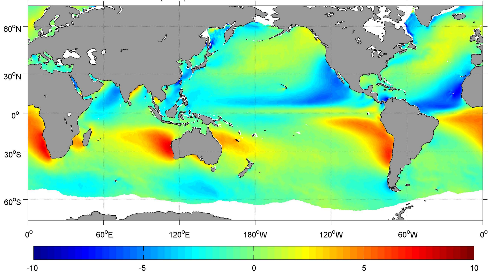
March SCOW Meridional Wind ( \text{m s}^{-1} )
