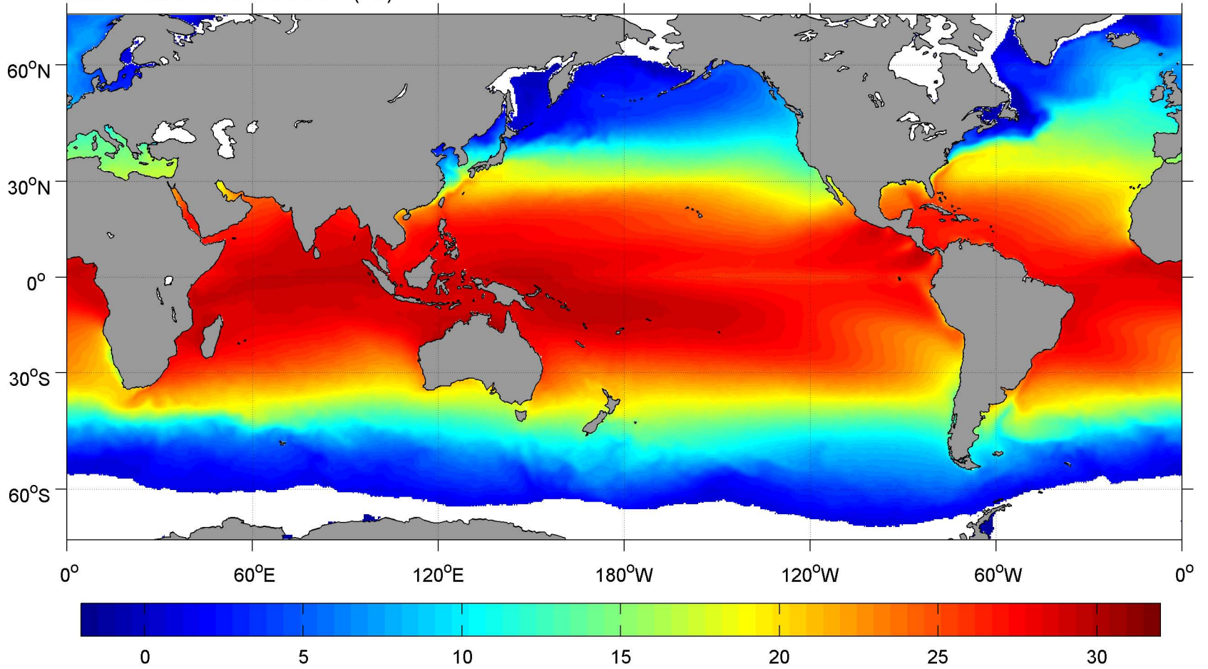
March SCOW AVHRR SST ( ^{\circ}\text{C} )
