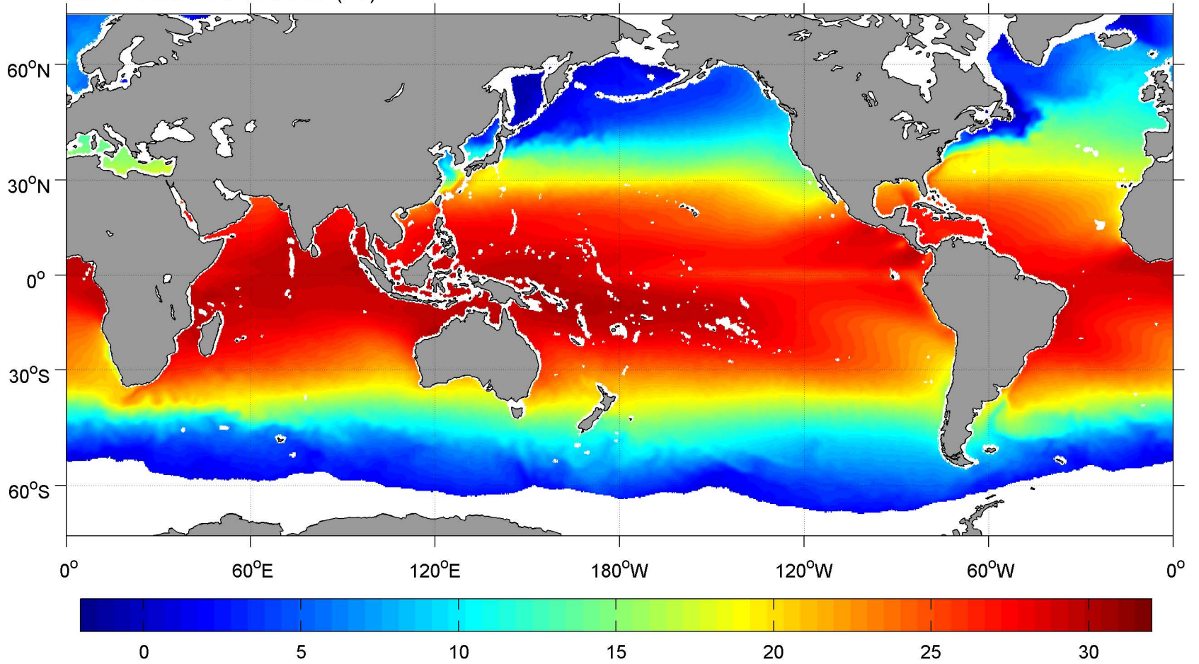
March SCOW AMSR SST ( ^{\circ}\text{C} )
