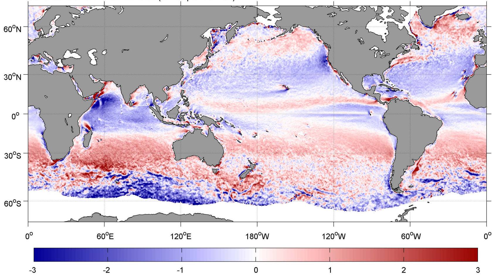
June SCOW Wind Stress Curl ( \text{N m}^{-2} per 10^4 \text{ km}^2 )
