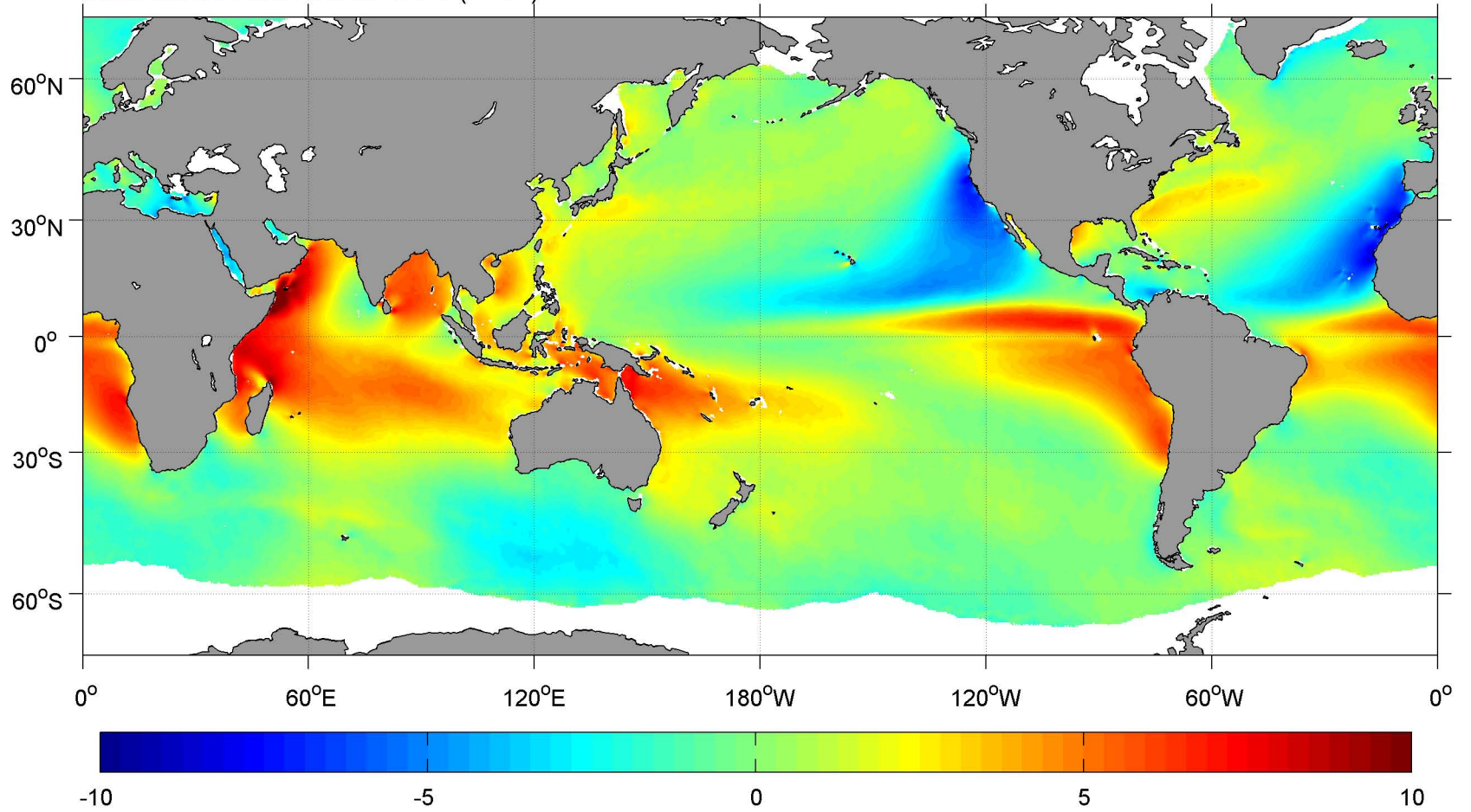
June SCOW Meridional Wind ( \text{m s}^{-1} )
