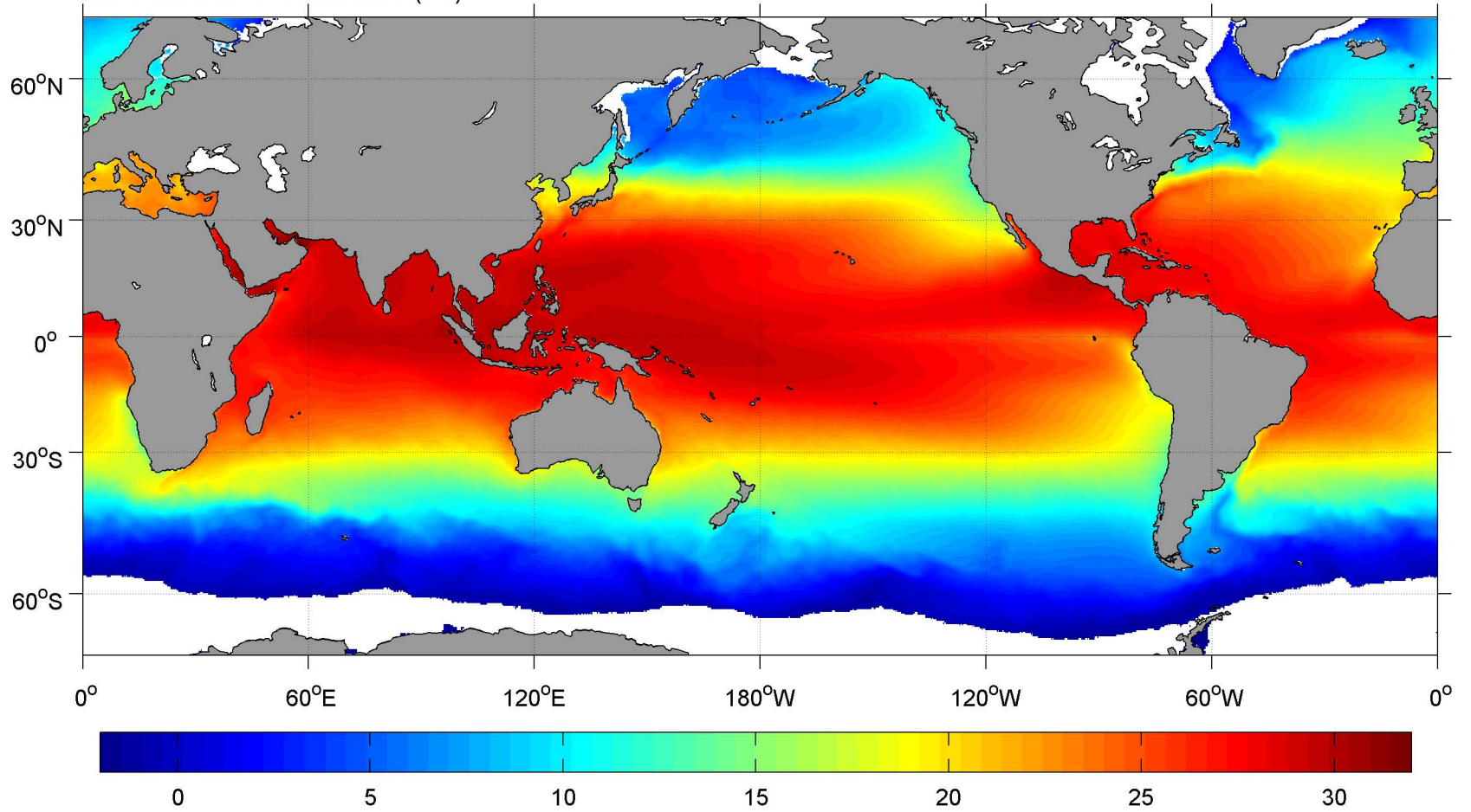
June SCOW AVHRR SST ( ^{\circ}\text{C} )
