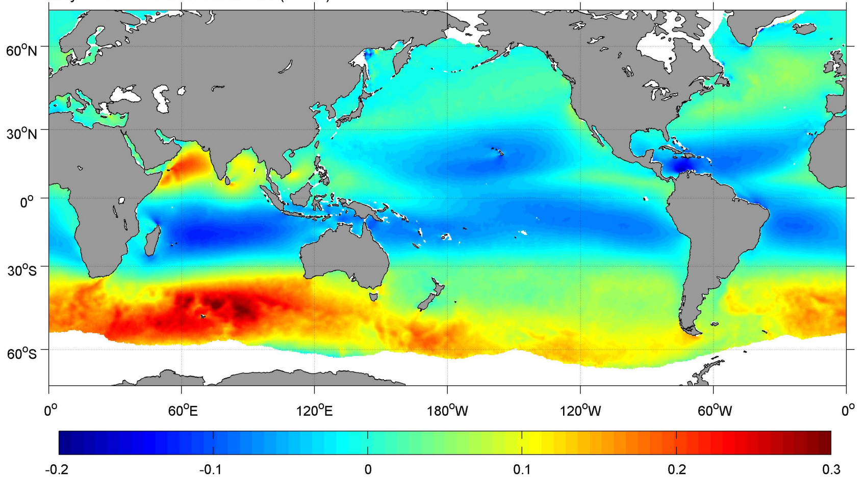
July SCOW Zonal Wind Stress ( \text{N m}^{-2} )
