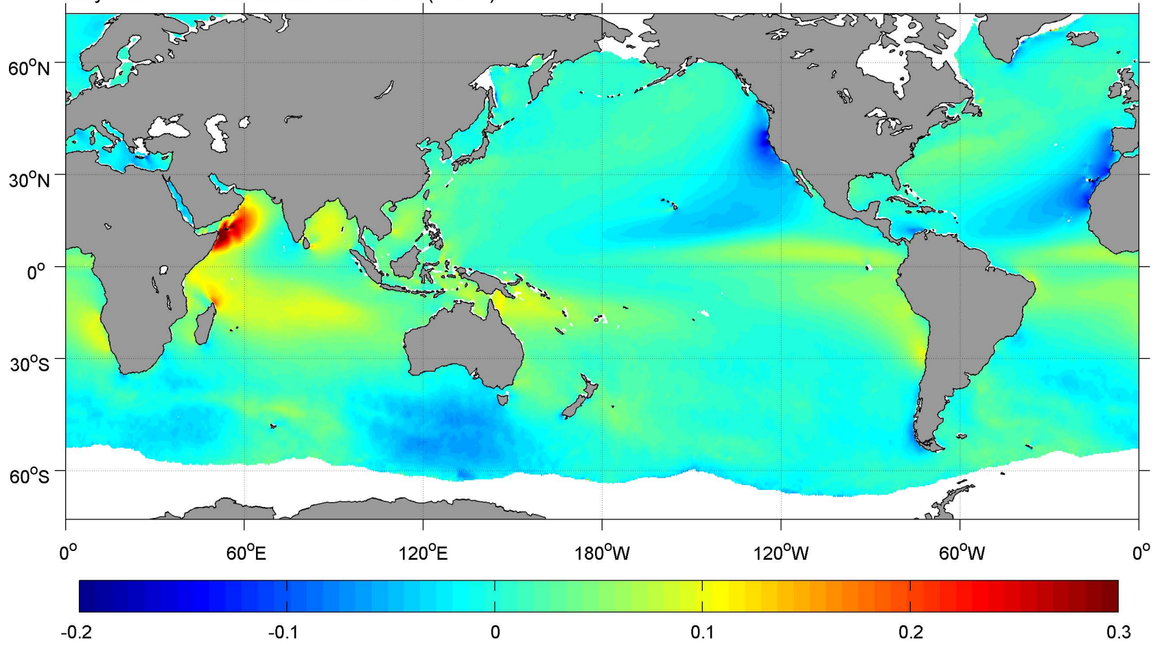
July SCOW Zonal Meridional Stress ( \text{N m}^{-2} )
