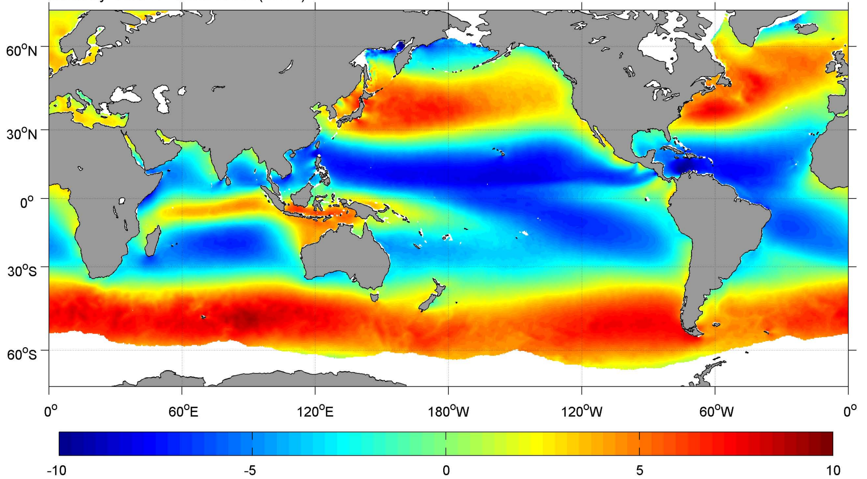
January SCOW Zonal Wind ( \text{m s}^{-1} )
