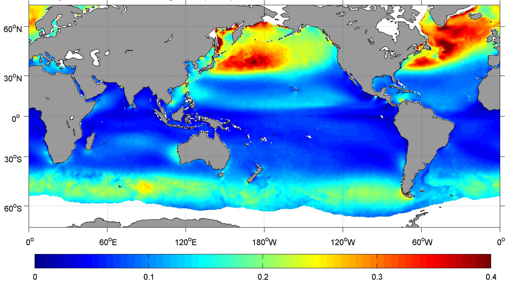
January SCOW Wind Stress Magnitude ( \text{N m}^{-2} )
