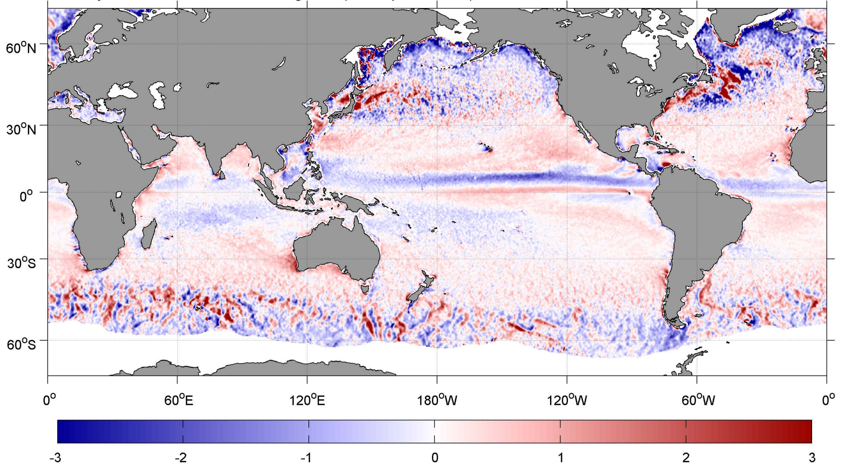
January SCOW Wind Stress Divergence ( \text{N m}^{-2} per 10^4 \text{ km}^2 )
