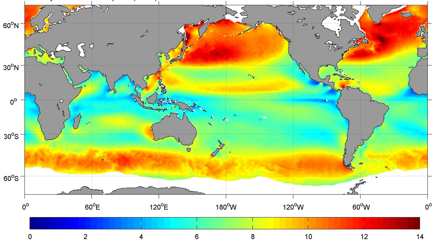
January SCOW Wind Speed ( \text{m s}^{-1} )
