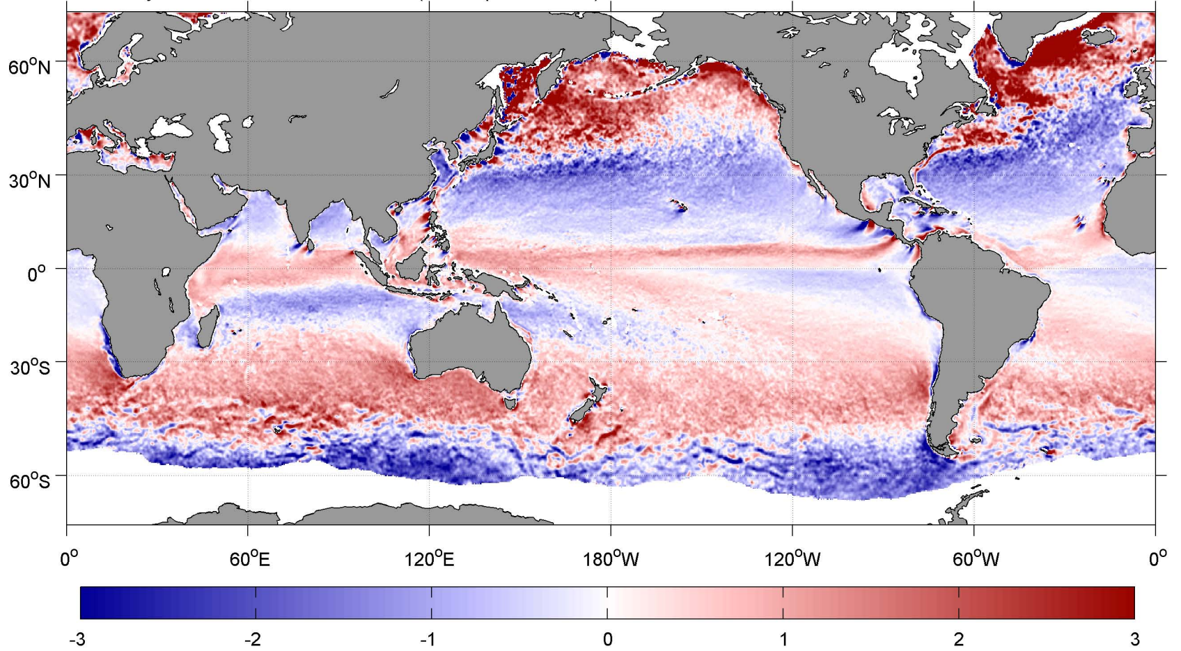
February SCOW Wind Stress Curl ( \text{N m}^{-2} per 10^4 \text{ km} )
