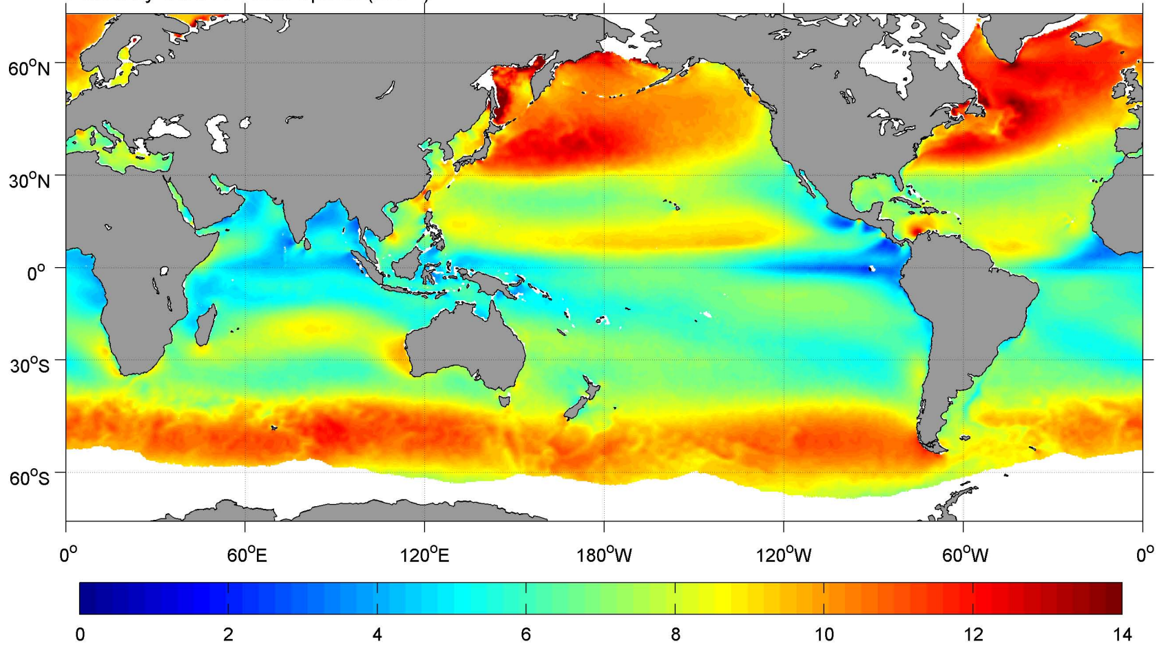
February SCOW Wind Speed ( \text{m s}^{-1} )
