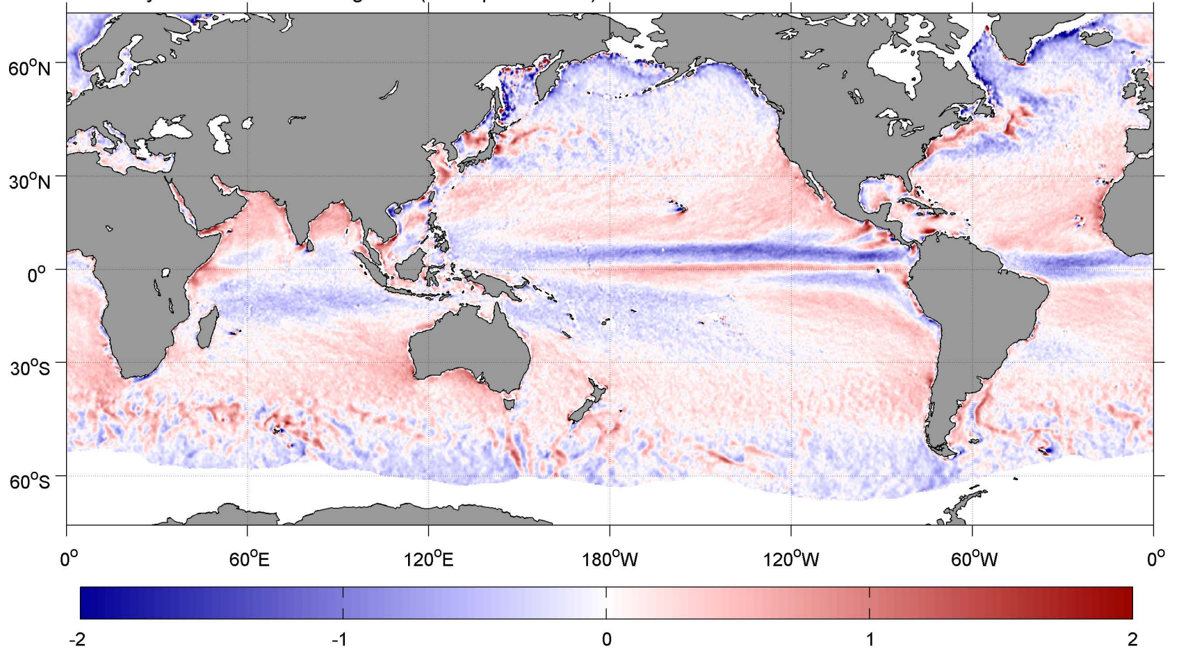
February SCOW Wind Divergence ( \text{m s}^{-1} per 10^2 \text{ km} )
