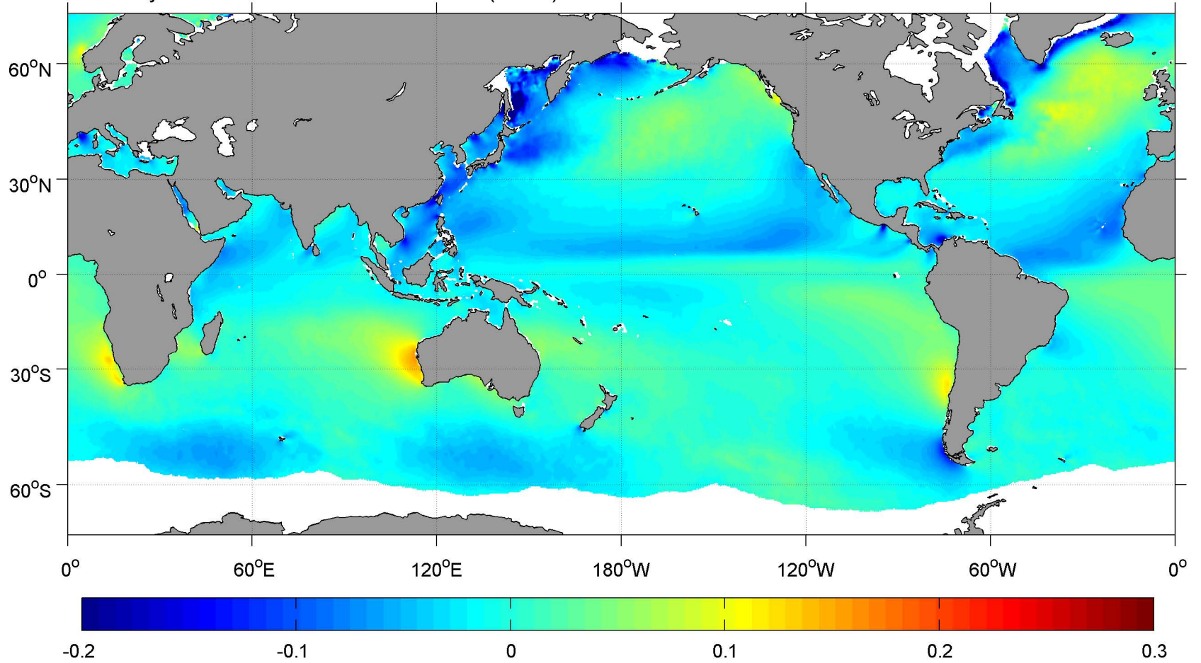
February SCOW Meridional Wind Stress ( \text{N m}^{-2} )
