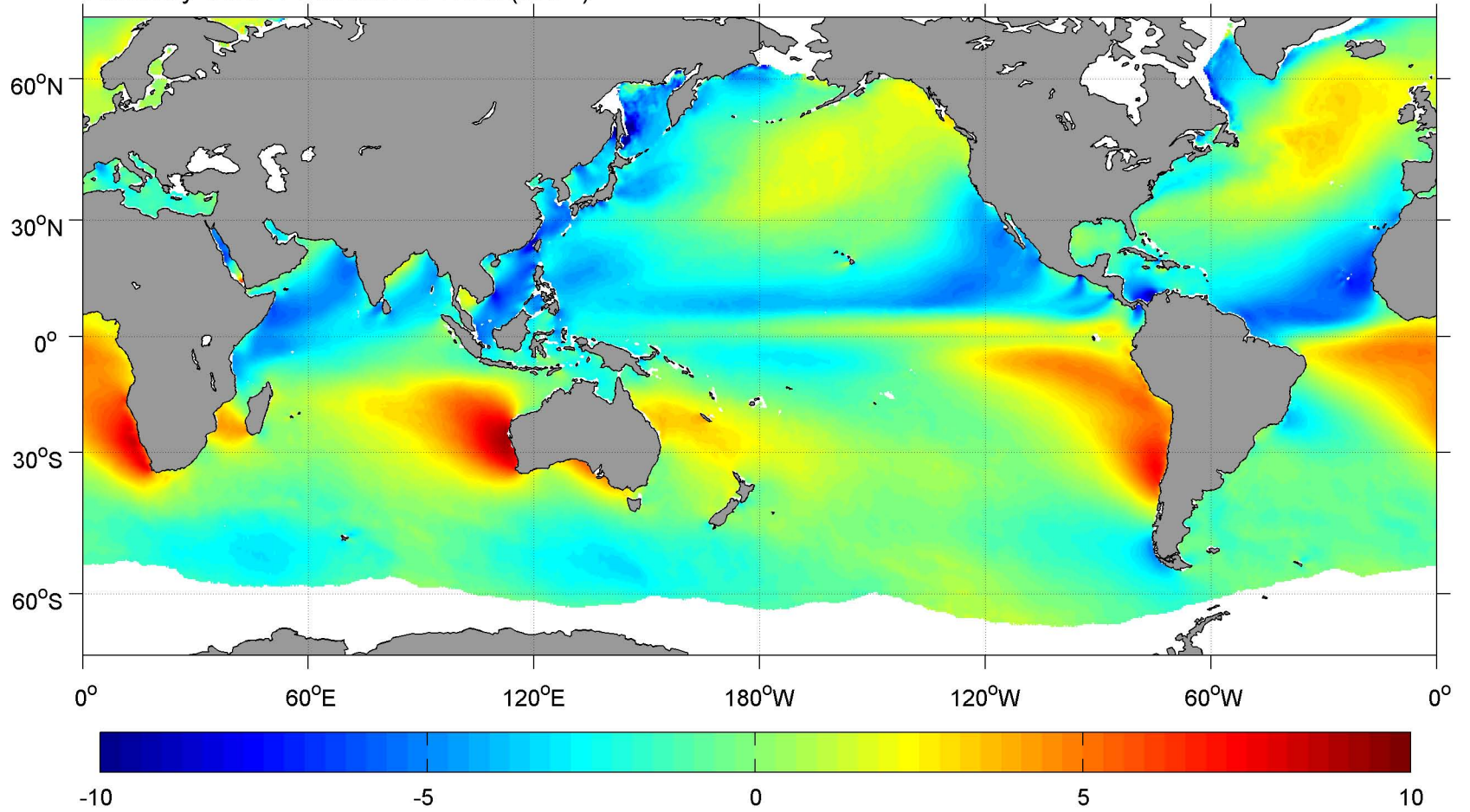
February SCOW Meridional Wind ( \text{m s}^{-1} )
