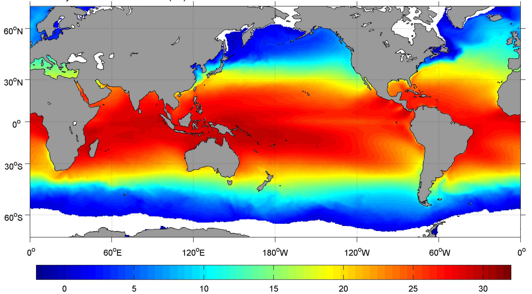
February SCOW AVHRR SST ( ^{\circ}\text{C} )
