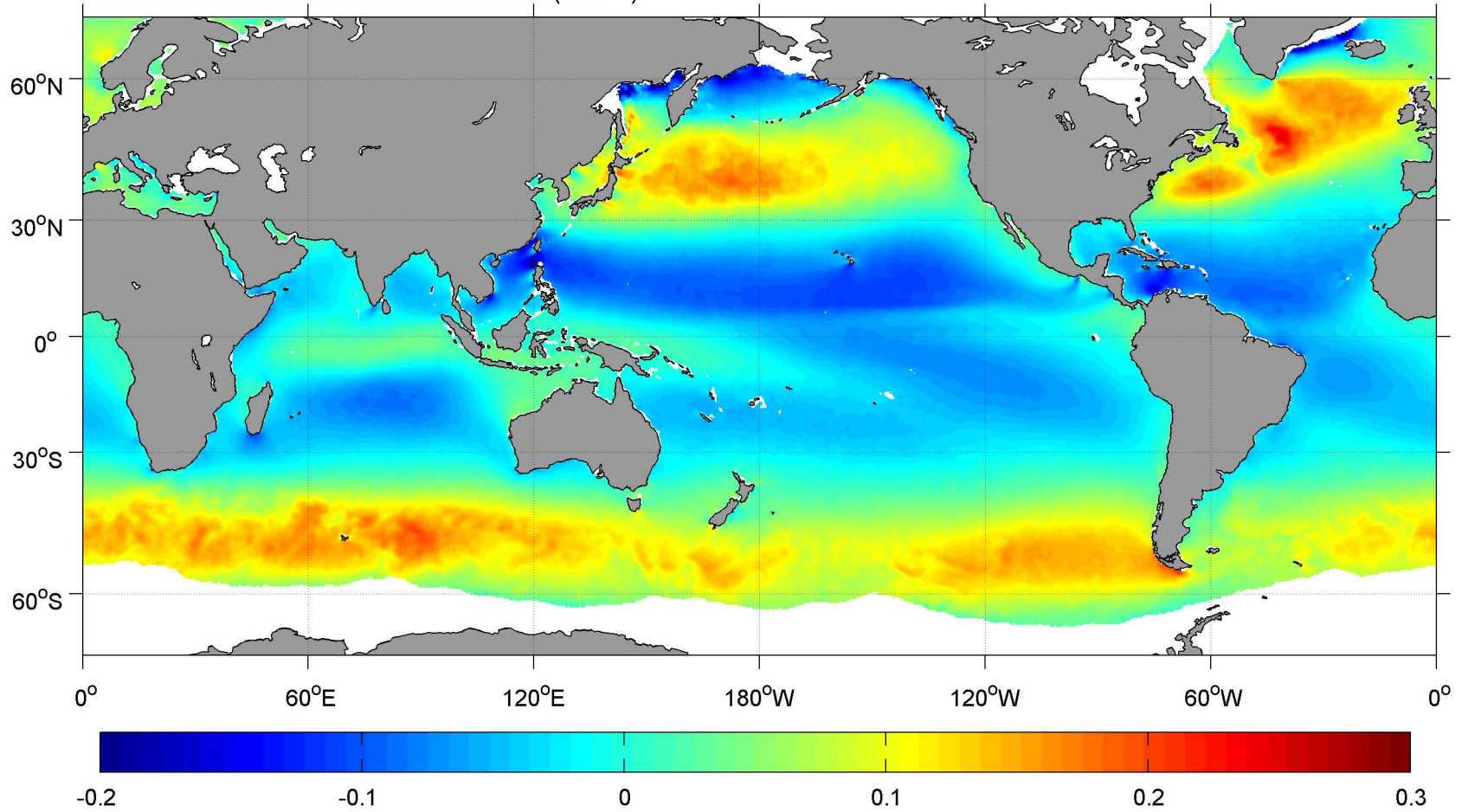
December SCOW Zonal Wind Stress ( \text{N m}^{-2} )
