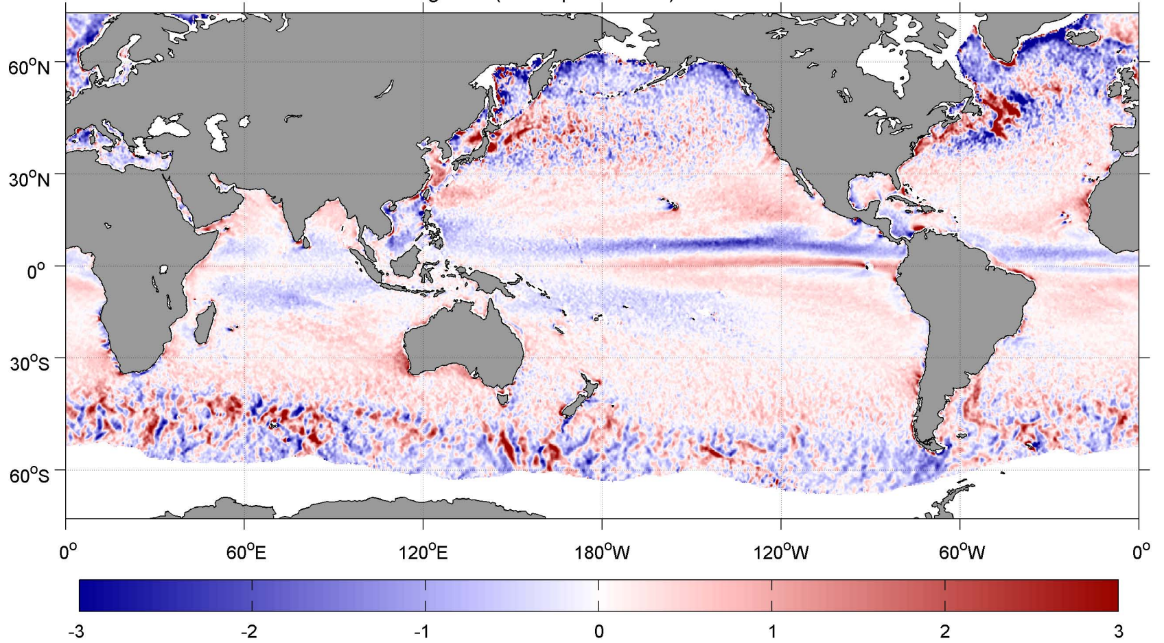
December SCOW Wind Stress Divergence ( \text{N m}^{-2} per 10^4 \text{ km}^2 )
