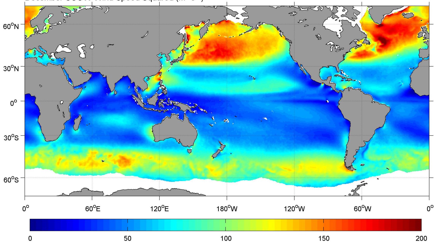
December SCOW Wind Speed Squared ( \text{m}^2 \text{s}^{-2} )
