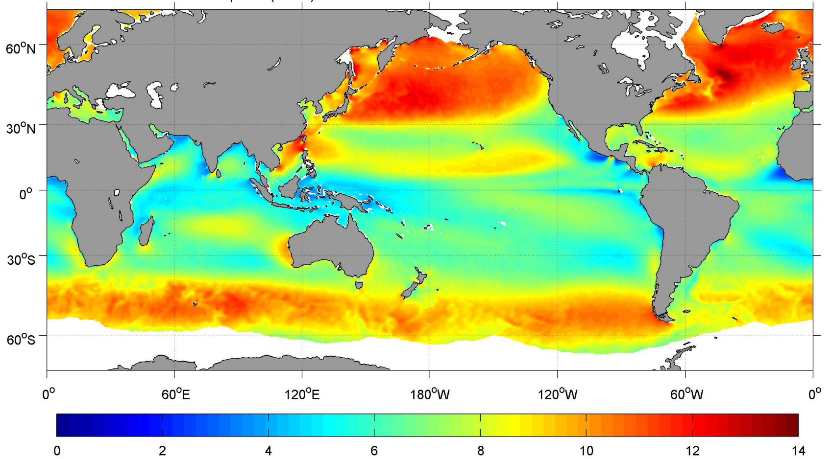
December SCOW Wind Speed ( \text{m s}^{-1} )
