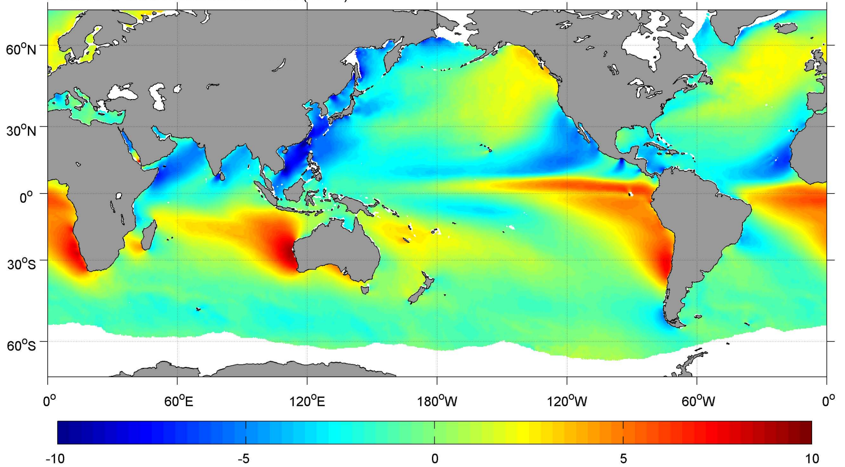
December SCOW Meridional Wind ( \text{m s}^{-1} )
