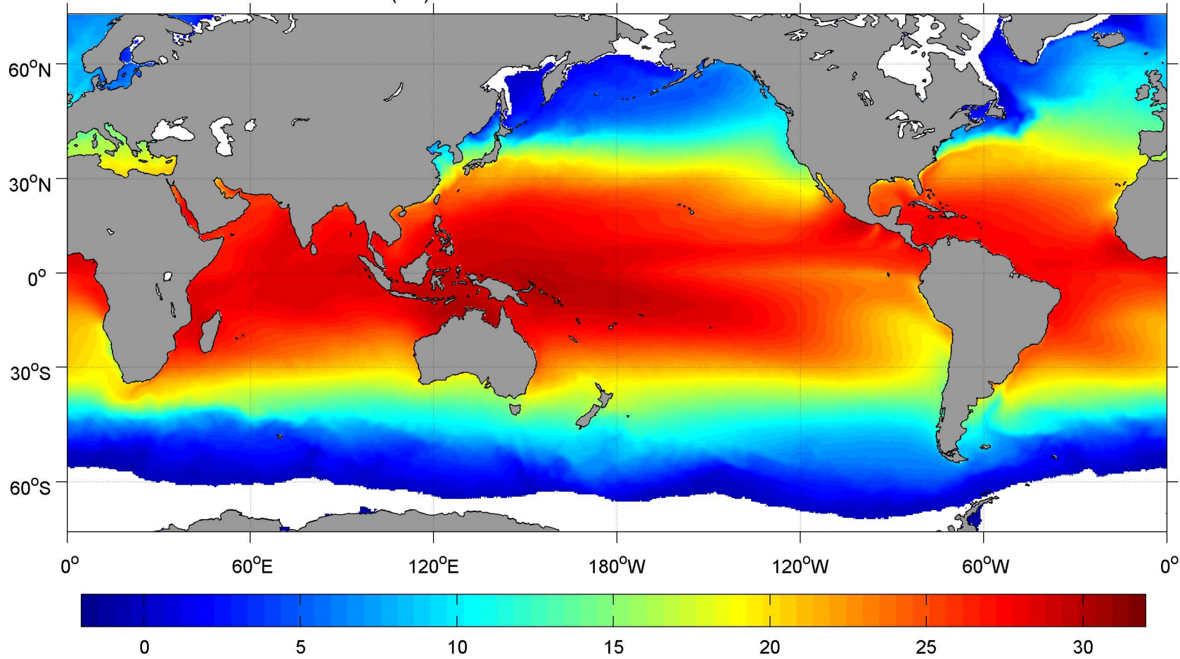
December SCOW AVHRR SST ( ^{\circ}\text{C} )
