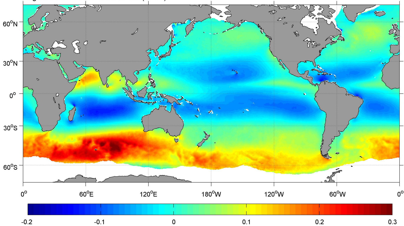
August SCOW Zonal Wind Stress ( \text{N m}^{-2} )
