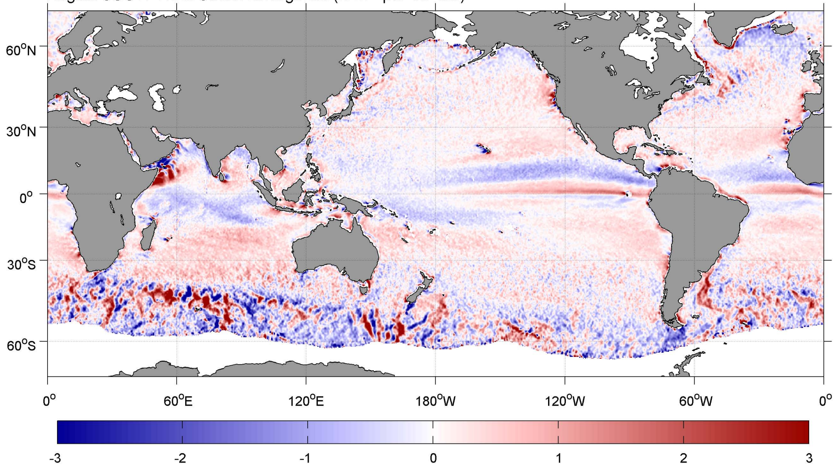
August SCOW Wind Stress Divergence ( \text{N m}^{-2} per 10^4 \text{ km}^2 )
