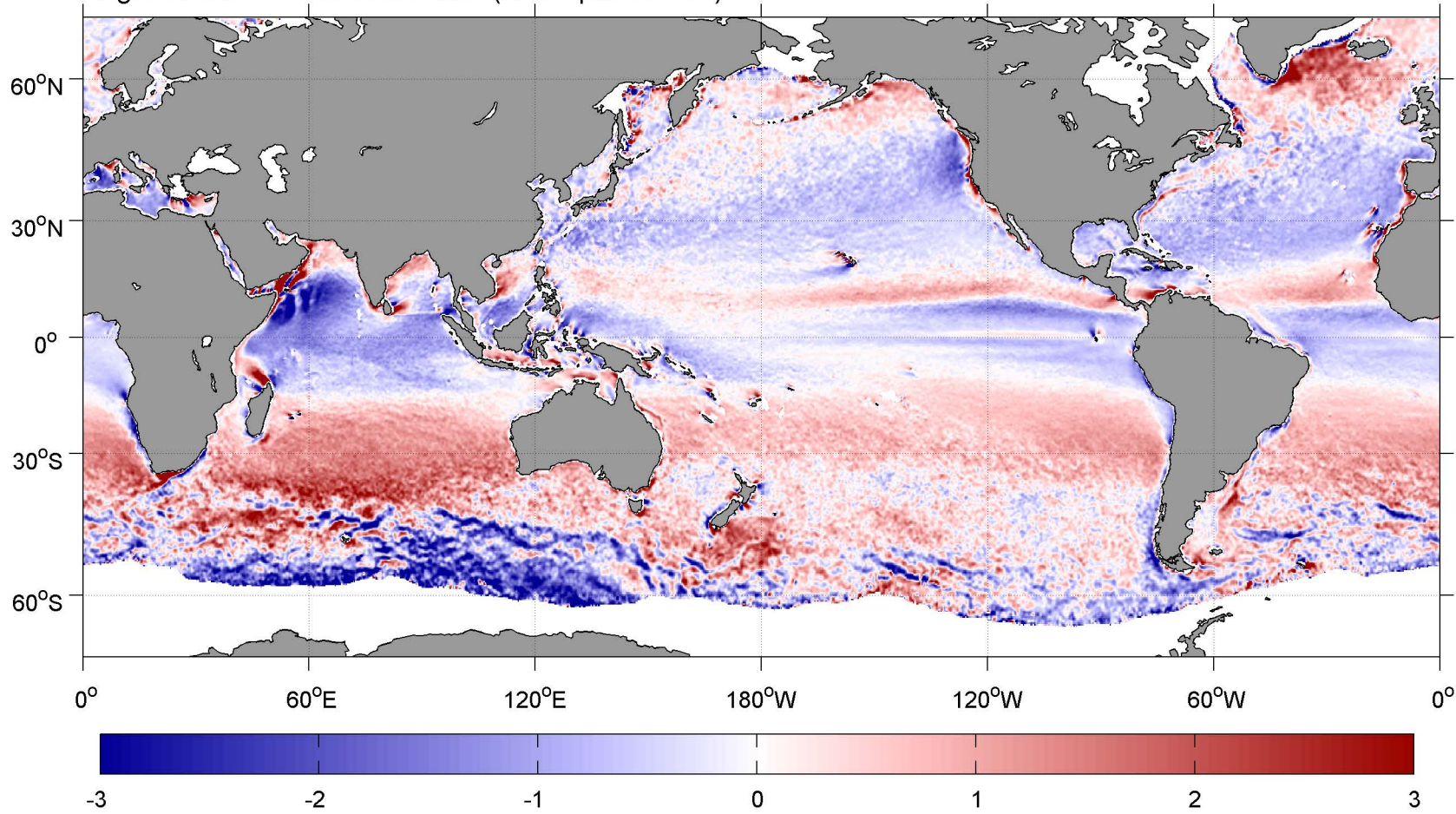
August SCOW Wind Stress Curl ( \text{N m}^{-2} per 10^4 \text{ km} )
