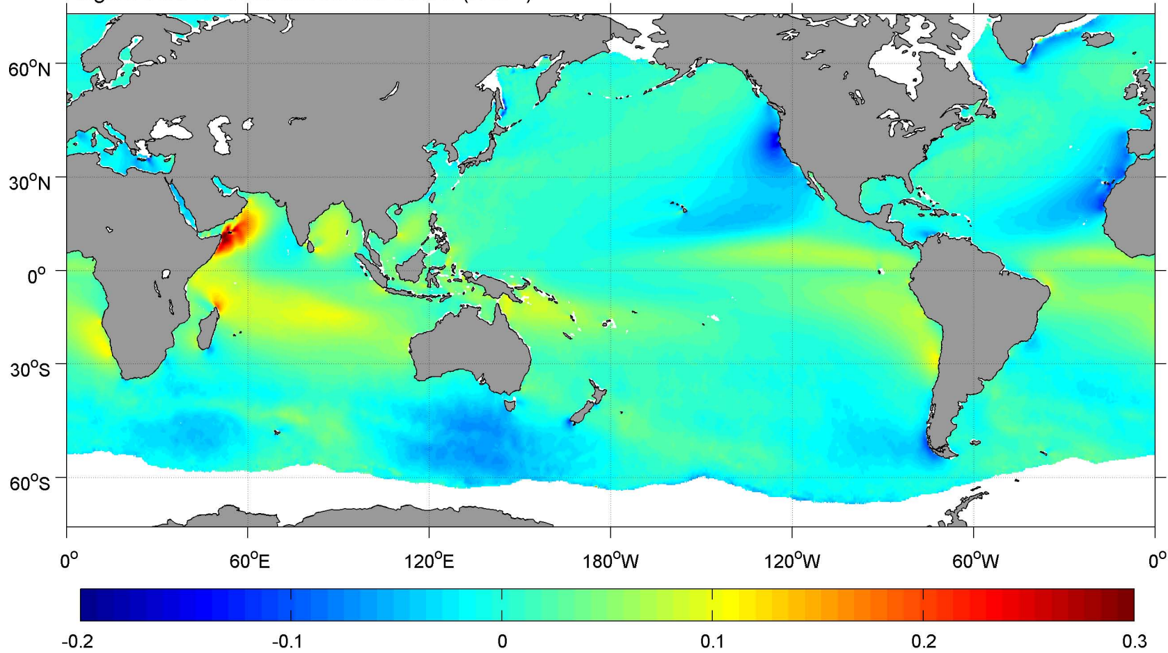
August SCOW Zonal Meridional Stress ( \text{N m}^{-2} )
