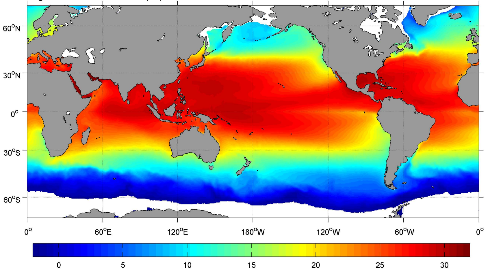
August SCOW AVHRR SST ( ^{\circ}\text{C} )
