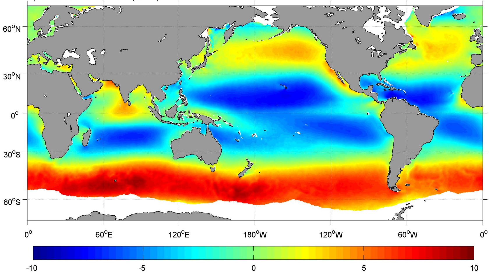
April SCOW Zonal Wind ( \text{m s}^{-1} )
