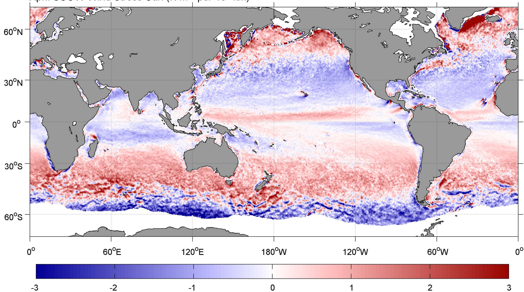
April SCOW Wind Stress Curl ( \text{N m}^{-2} per 10^4 \text{ km} )
