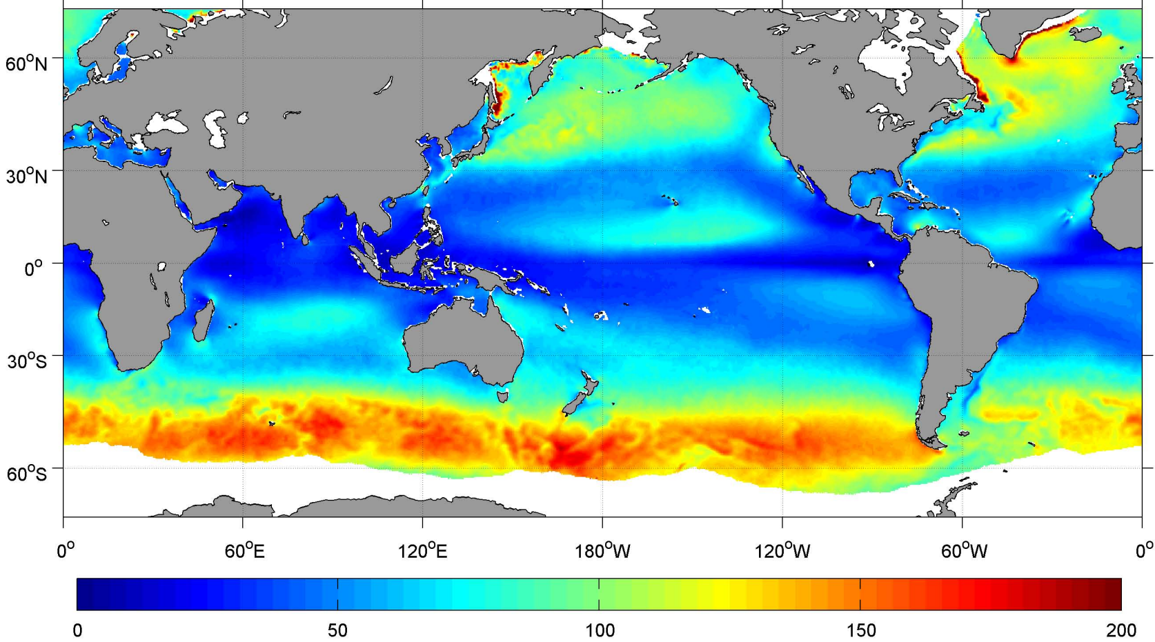
April SCOW Wind Speed Squared ( \text{m}^2 \text{s}^{-2} )
