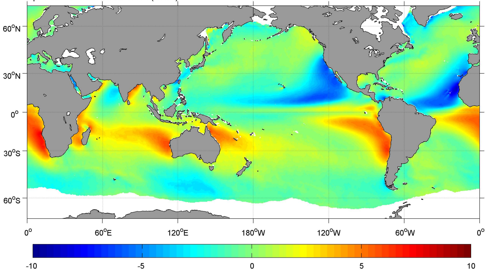
April SCOW Meridional Wind ( \text{m s}^{-1} )
